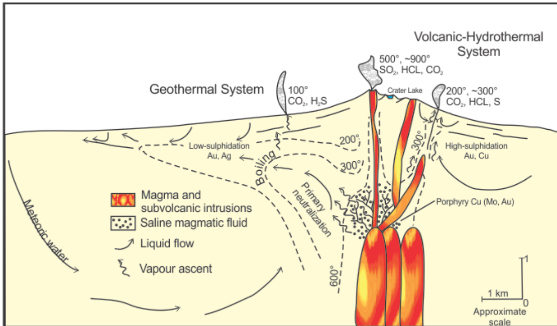
Figure 2a: Schematic cross section through an intrusive centered hydrothermal system outlining the environments of porphyry, high-sulphidation and low-sulphidation systems (Hedenquist and Lowenstern, 1994).
