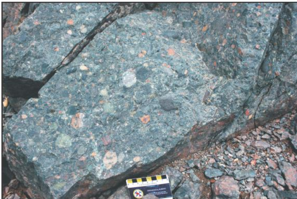
Plate 8: Pebble conglomerate of the Rocky Harbour Formation; Stop #1.5.
