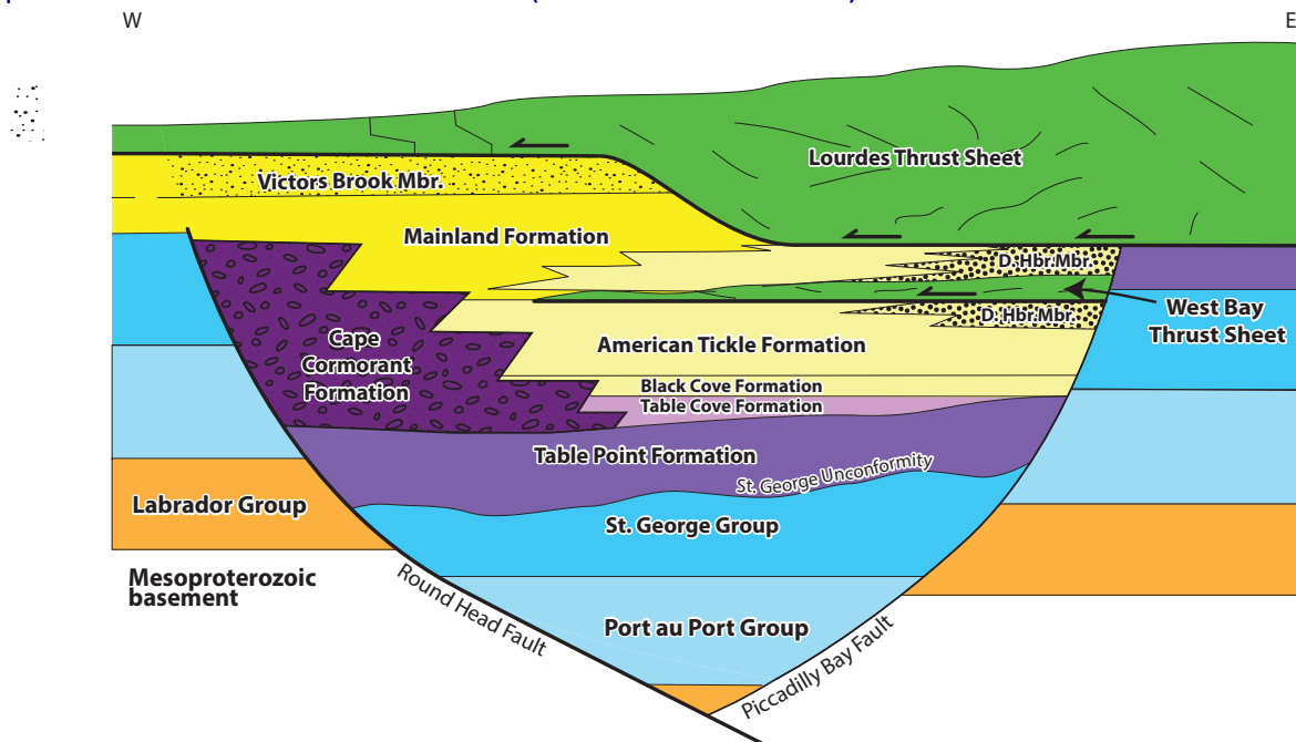
Figure 11 Schematic diagram of stratigraphic relationships in the faulted foreland basin preserved on Port au Port Peninsula (Lacombe et al. 2019b).
