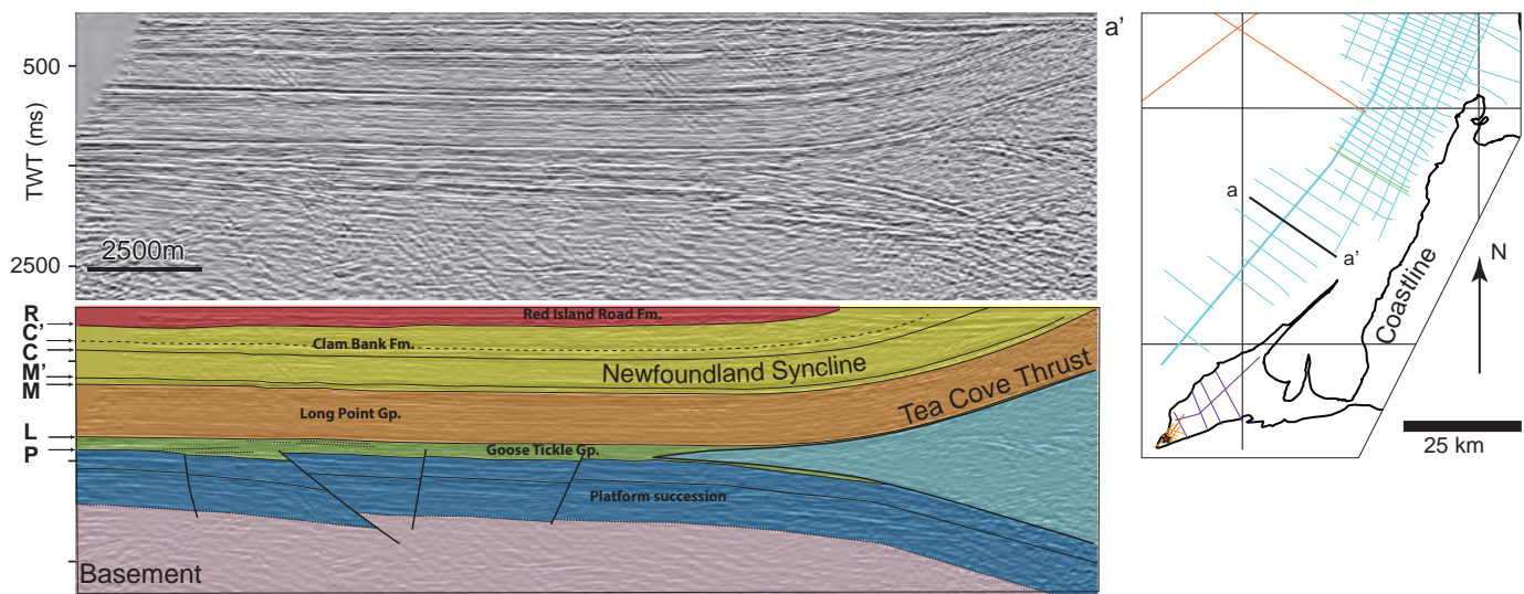
Figure 13: Seismic profile offshore of western Newfoundland (White et al. 2019a).
