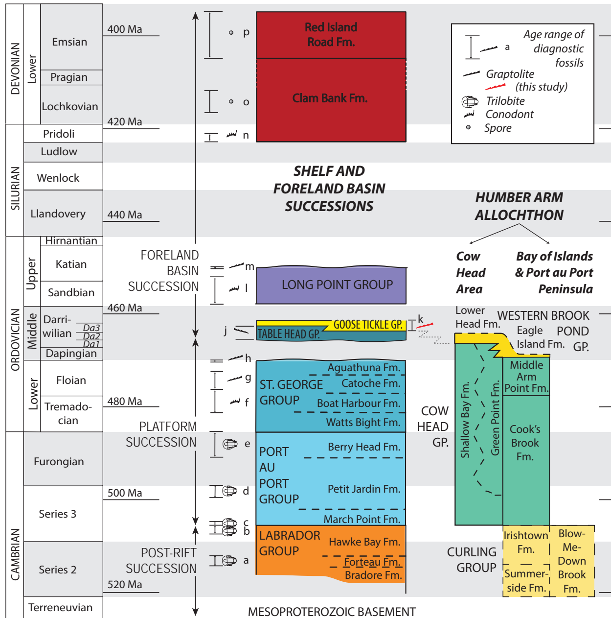
Figure 4 Stratigraphic columns for major units of Laurentian margin (Lacombe et al. 2019b).
