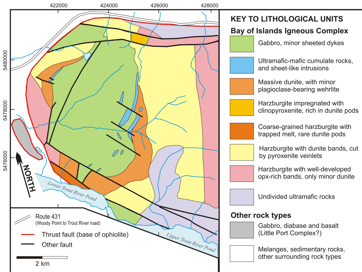
Figure 22: Schematic geologic map of the Tablelands (Kerr 2019)
