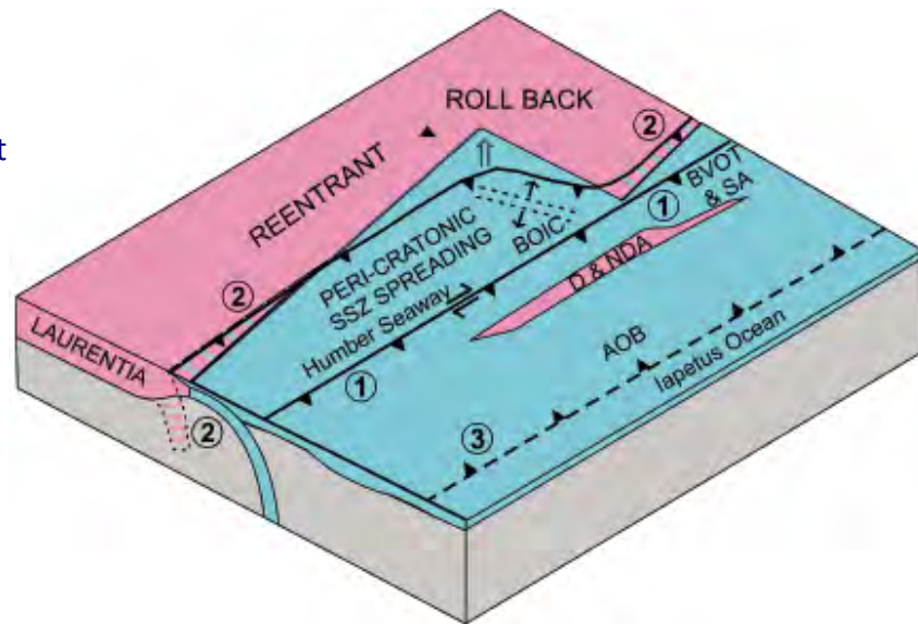
Figure 10 Scenario for spreading of the Bay of Islands ophiolite within the developing Taconian orogen at a re-entrant in the Laurentian margin, after van Staal et al. (2007)
