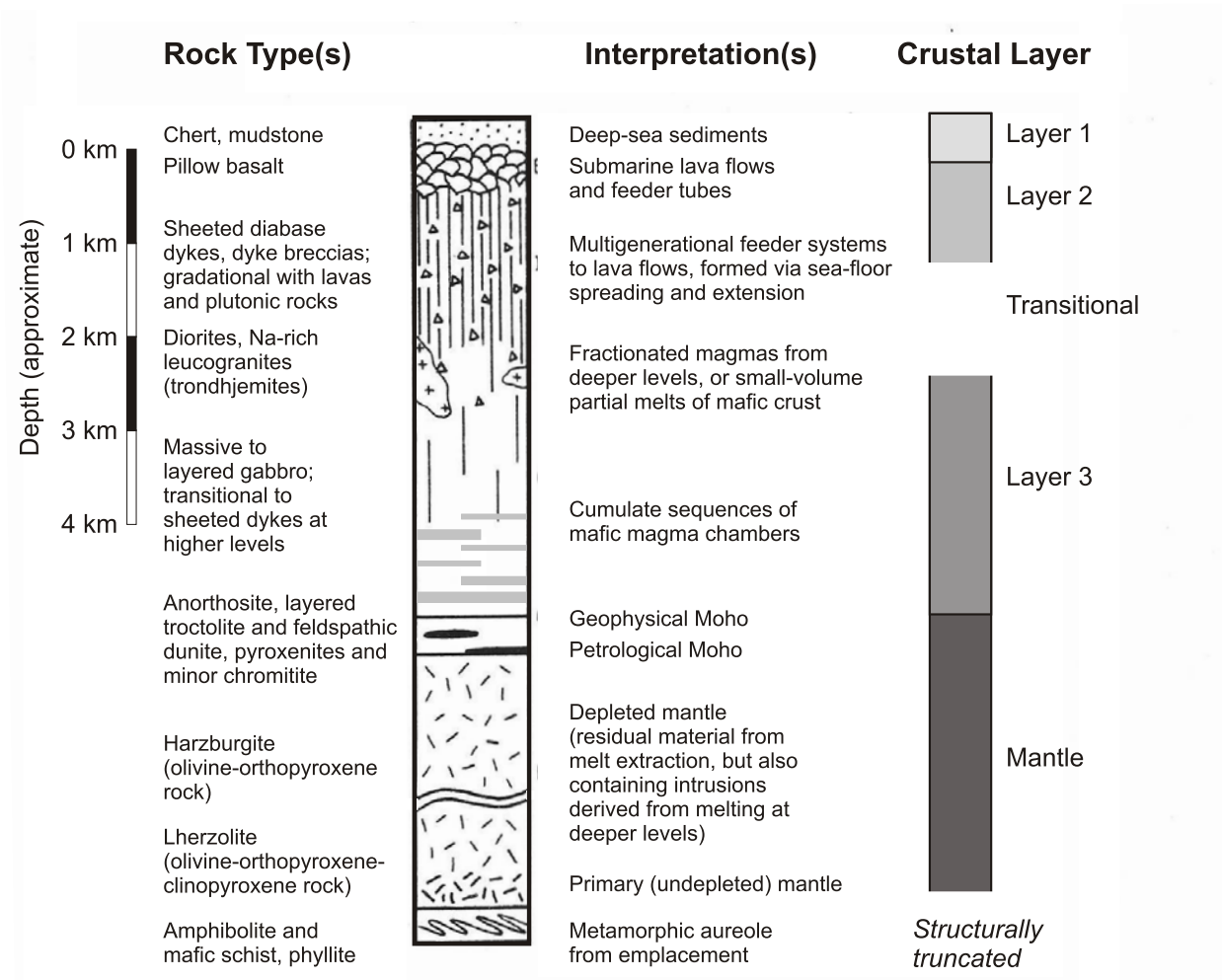
Figure 9 Subdivisions of an ideal ophiolite suite (Kerr 2019)
