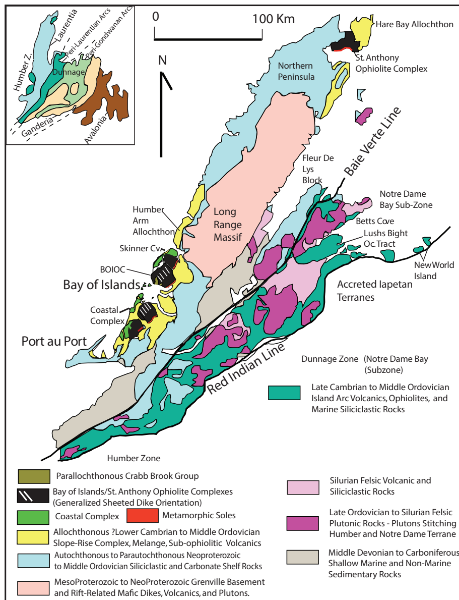
Figure 7 Map of western Newfoundland showing the principal ophiolitic units, after Dewey and Casey (2013)
