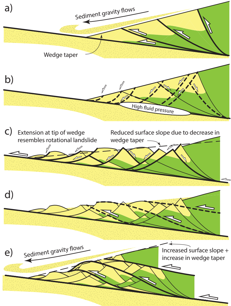
Figure 16: Development of broken formation and mélangé in an accretionary wedge or thrust belt subject to fluid-pressure variation (Lacombe et al. 2019a)
