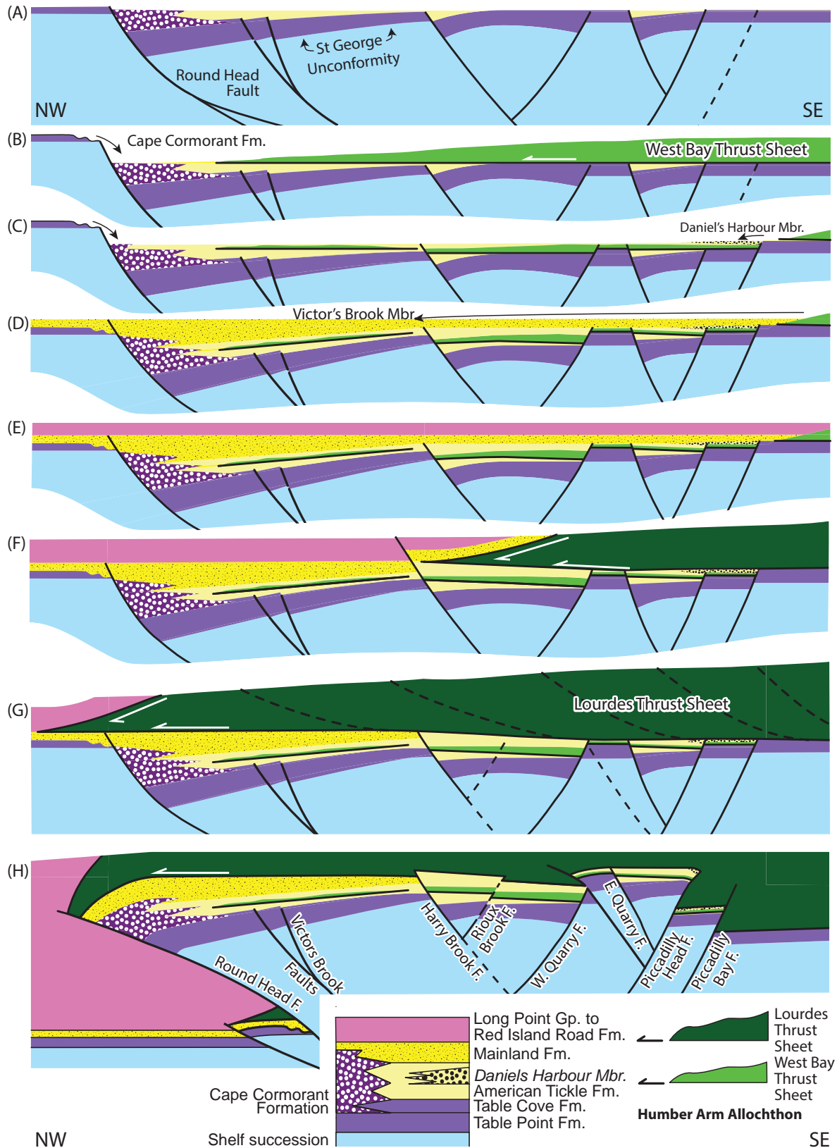
Figure 28: Schematic diagram showing faulting history of Port au Port Peninsula.
